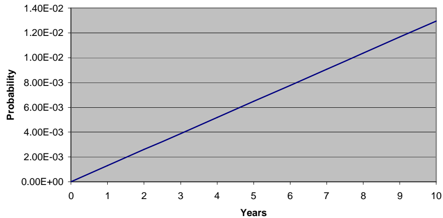
Figure 1: PFD AVG (t) 8800C Vortex Flowmeter
